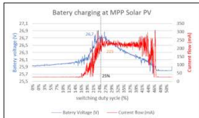
Figure 5: Battery voltage and current performance at optimum duty cycle 25%.
