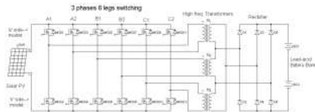
Figure 1: Lay out 3 phases 6 legs dc/dc converter for solar PV battery charging
