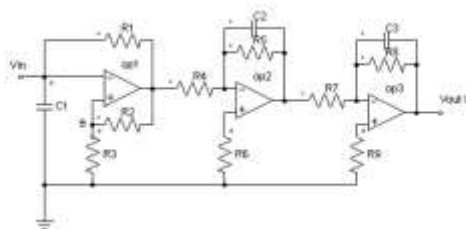
Figure 2: Sine wave generator circuit
