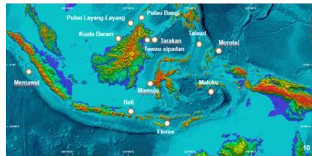
Figure 2: OTEC survey in Malaysia and Indonesia [Koto 2017 & UTM OTEC, 2017]
