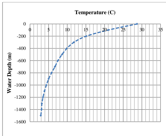
Figure 5: Sea Surface Temperature Data in Layang-Layang, Island, Sabah [1].
